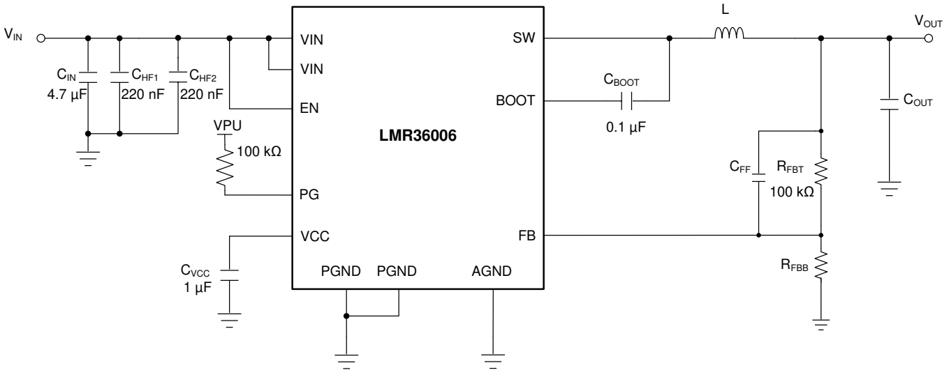
Figure 18. Example Applications Circuit
