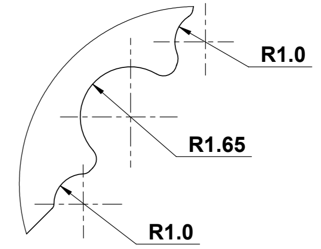
DETAIL B SCALE 8 : 1 (2 Places)
