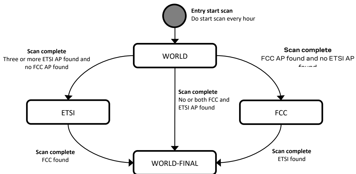
Figure 2: ODIN-W2 series IEEE 802.11d state transition diagram
